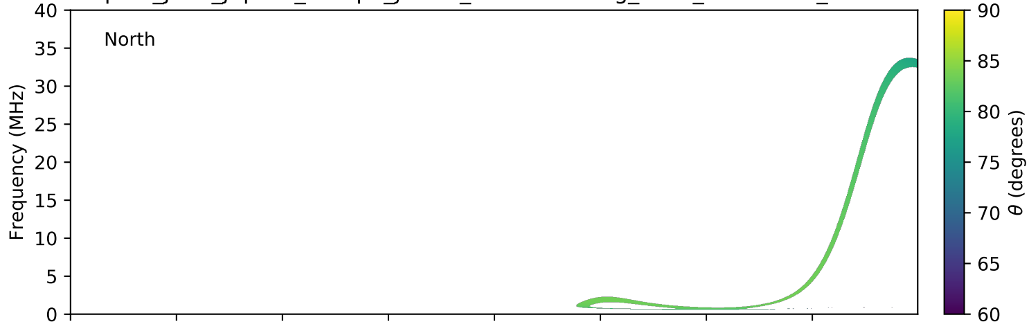
expres_juno_jupiter_europa_jrm09_lossc-wid1deg_3kev_20191018_v01.cdf
