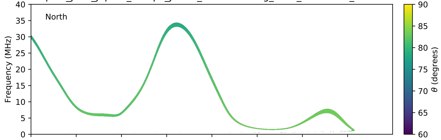
expres_juno_jupiter_europa_jrm09_lossc-wid1deg_3kev_20191012_v01.cdf
