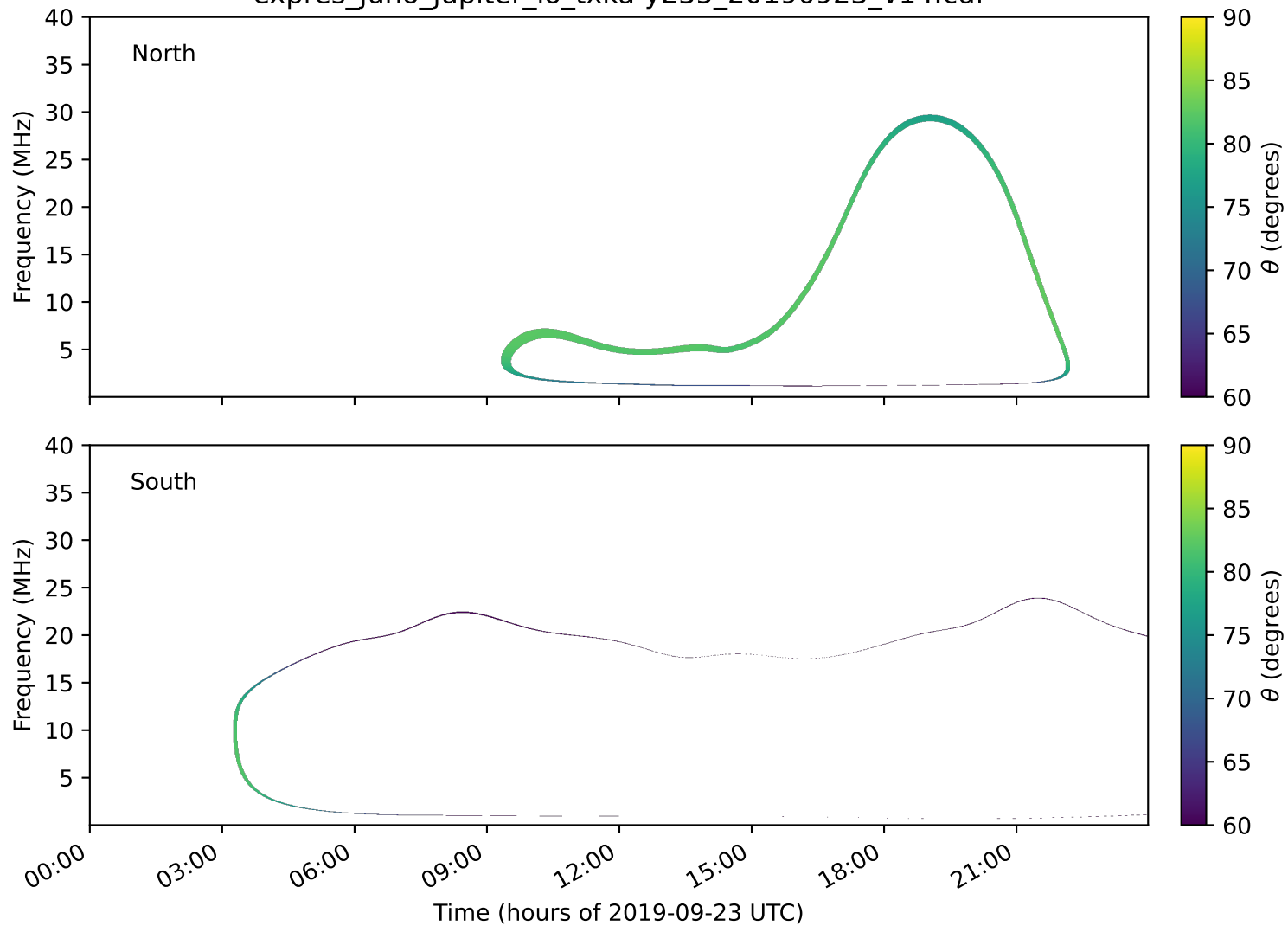
expres_juno_jupiter_io_txka-y235_20190923_v14.cdf
