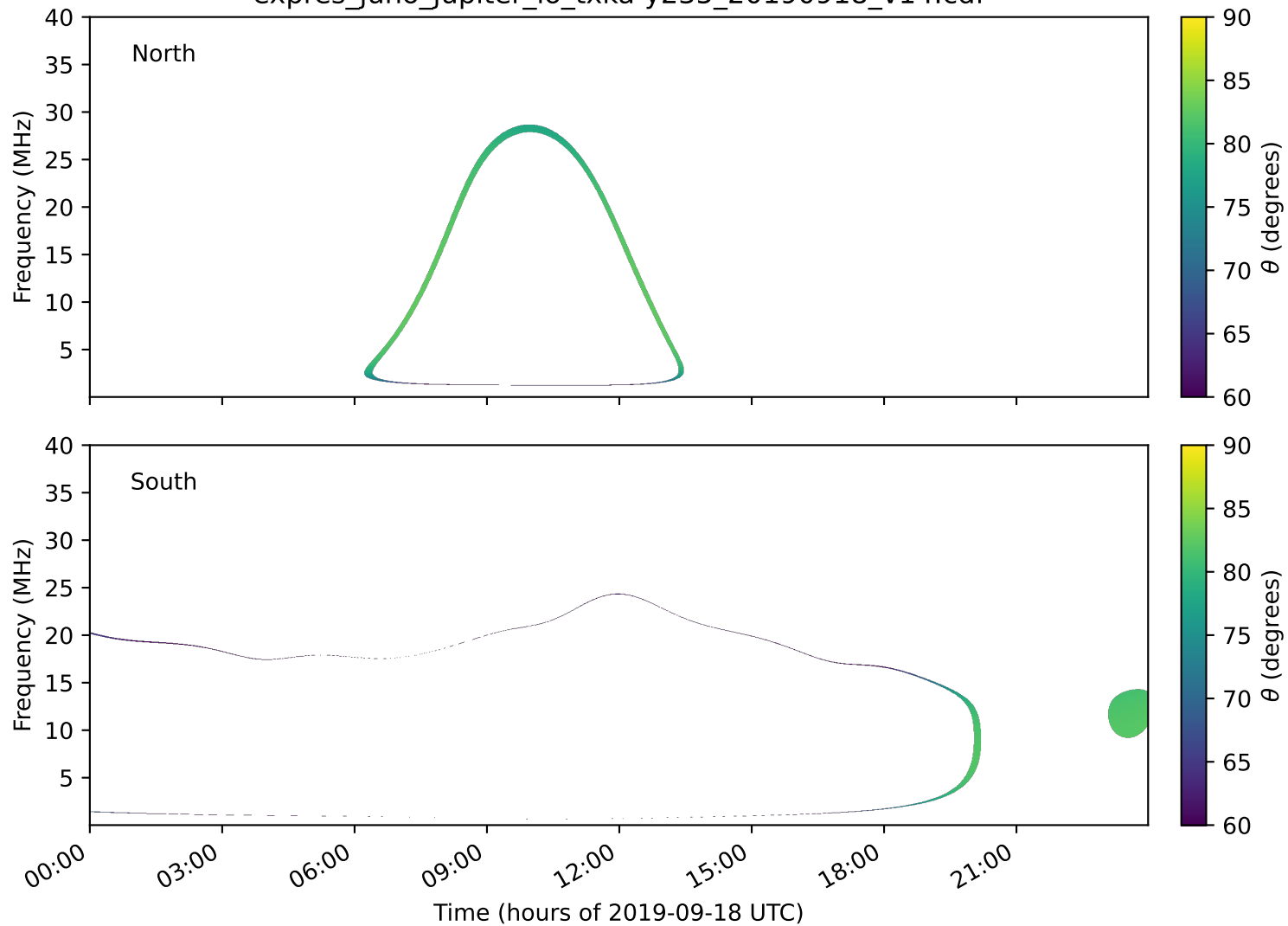
expres_juno_jupiter_io_txka-y235_20190918_v14.cdf
