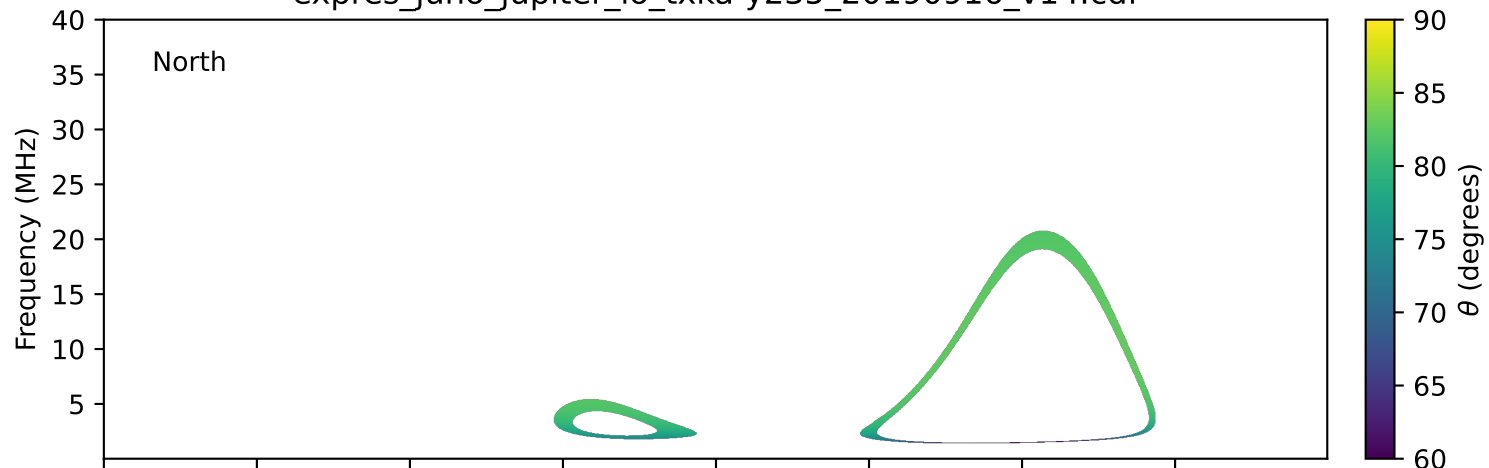
expres_juno_jupiter_io_txka-y235_20190916_v14.cdf
