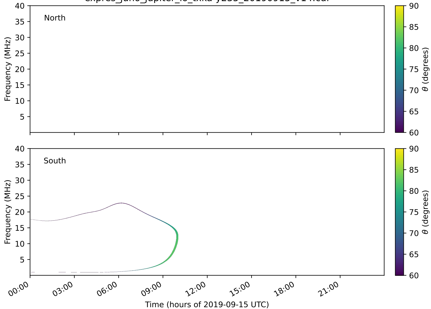
expres_juno_jupiter_io_txka-y235_20190915_v14.cdf
