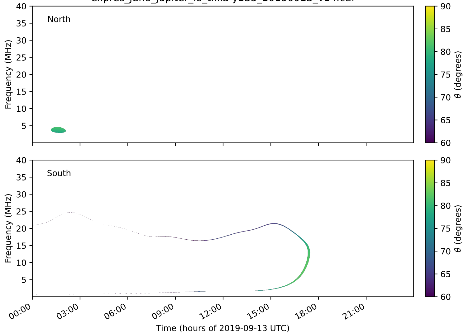
expres_juno_jupiter_io_txka-y235_20190913_v14.cdf
