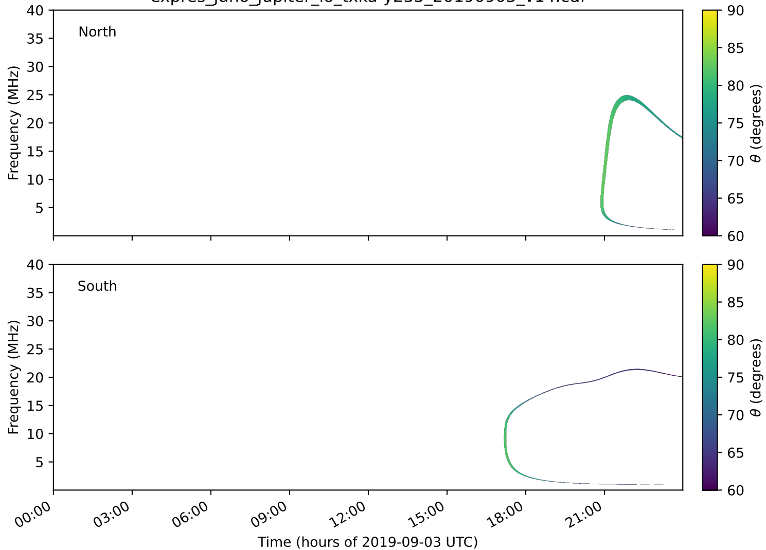
expres_juno_jupiter_io_txka-y235_20190903_v14.cdf
