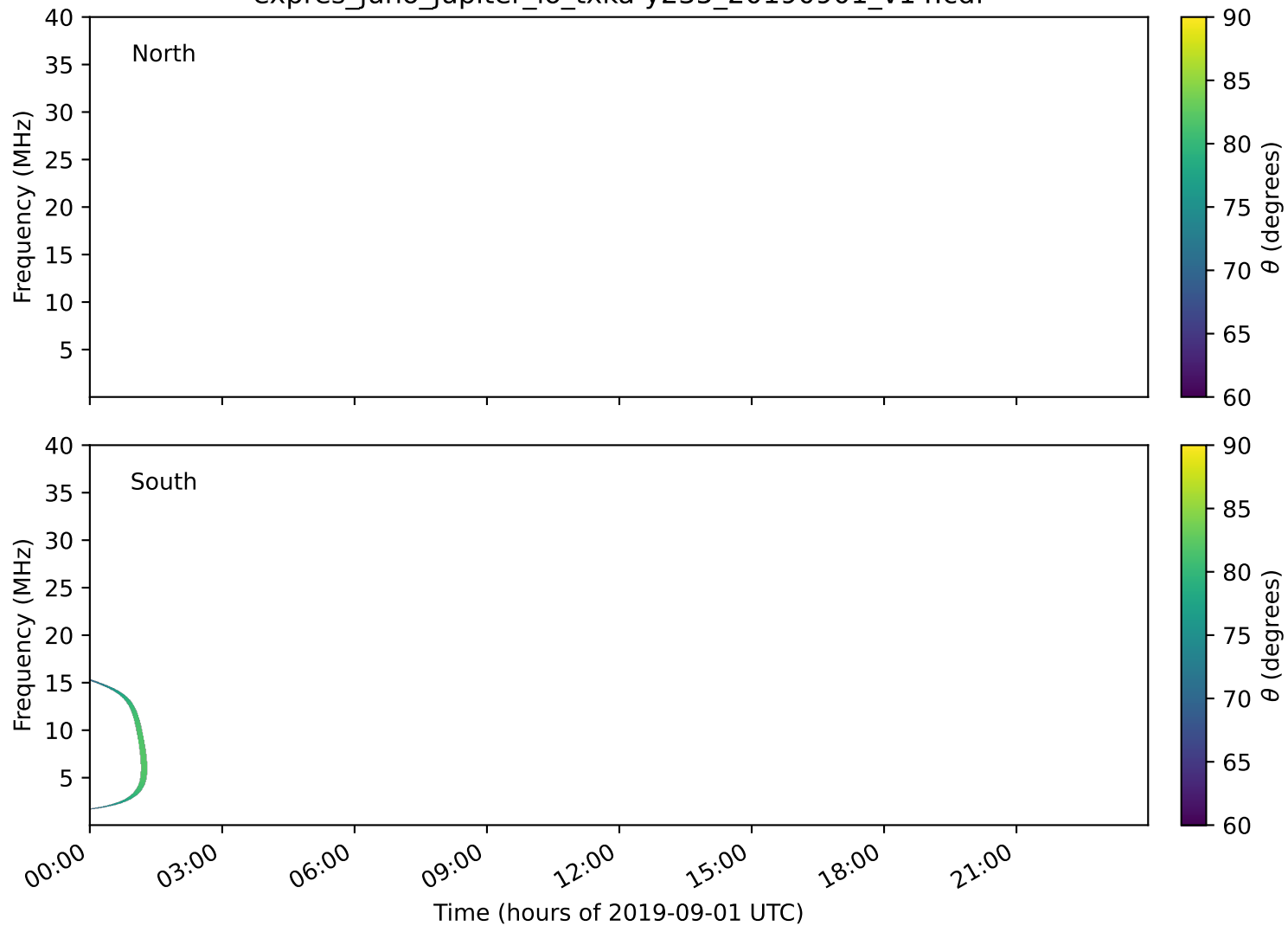
expres_juno_jupiter_io_txka-y235_20190901_v14.cdf
