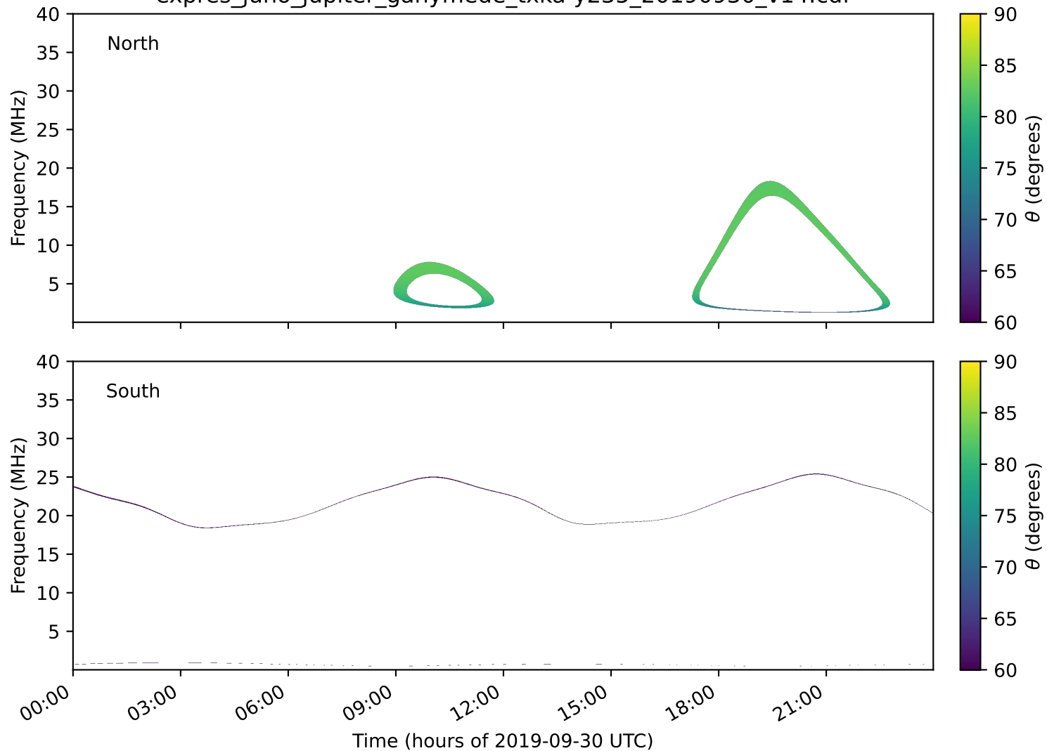
expres_juno_jupiter_ganymede_txka-y235_20190930_v14.cdf
