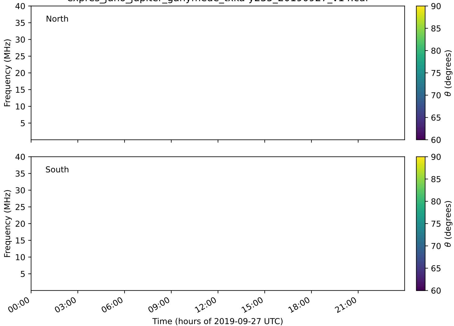
expres_juno_jupiter_ganymede_txka-y235_20190927_v14.cdf
