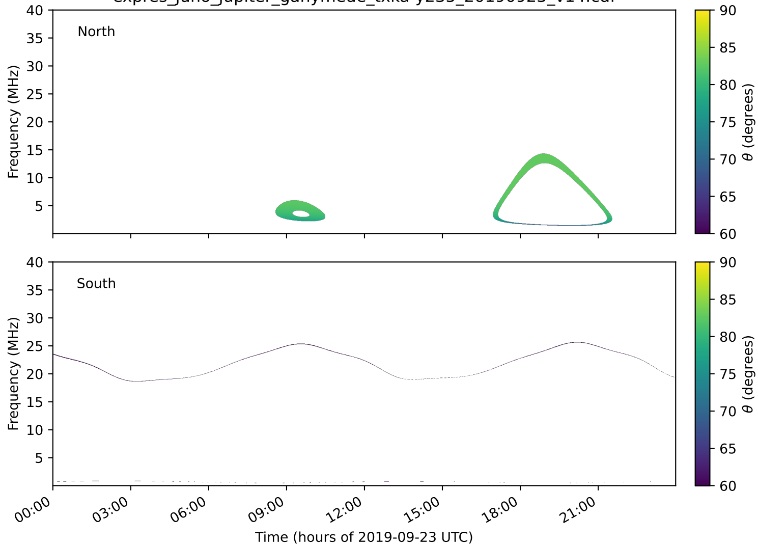
expres_juno_jupiter_ganymede_txka-y235_20190923_v14.cdf
