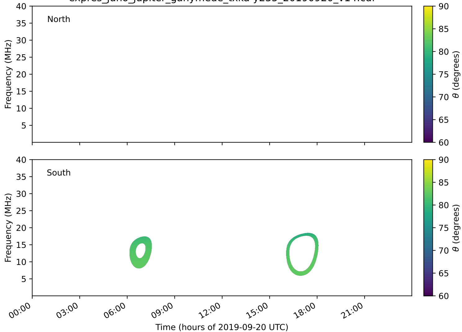
expres_juno_jupiter_ganymede_txka-y235_20190920_v14.cdf
