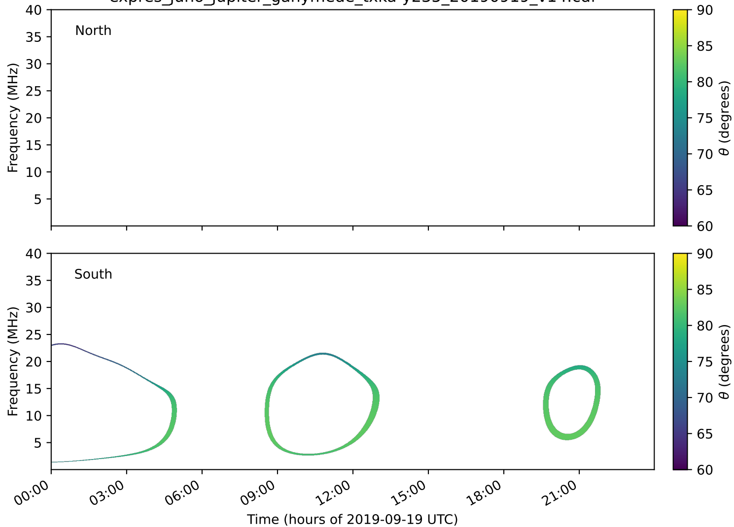
expres_juno_jupiter_ganymede_txka-y235_20190919_v14.cdf
