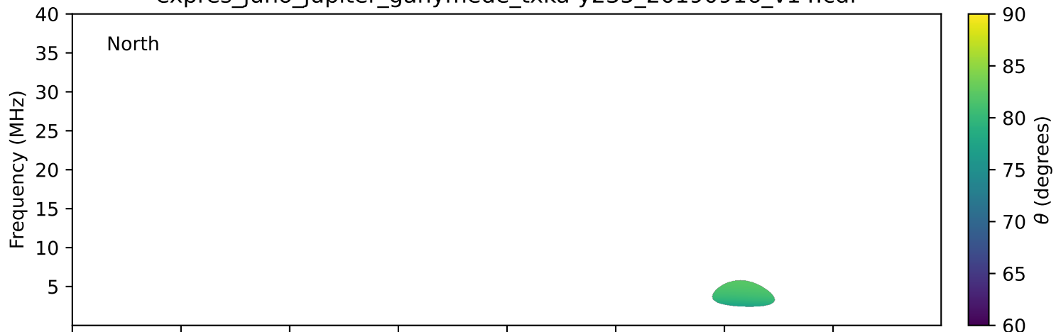
expres_juno_jupiter_ganymede_txka-y235_20190916_v14.cdf
