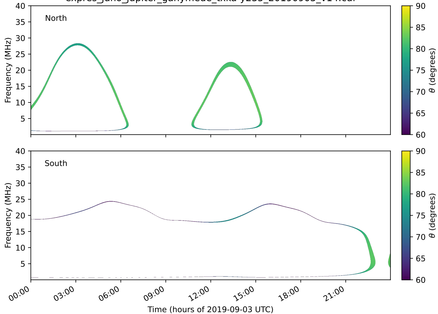
expres_juno_jupiter_ganymede_txka-y235_20190903_v14.cdf
