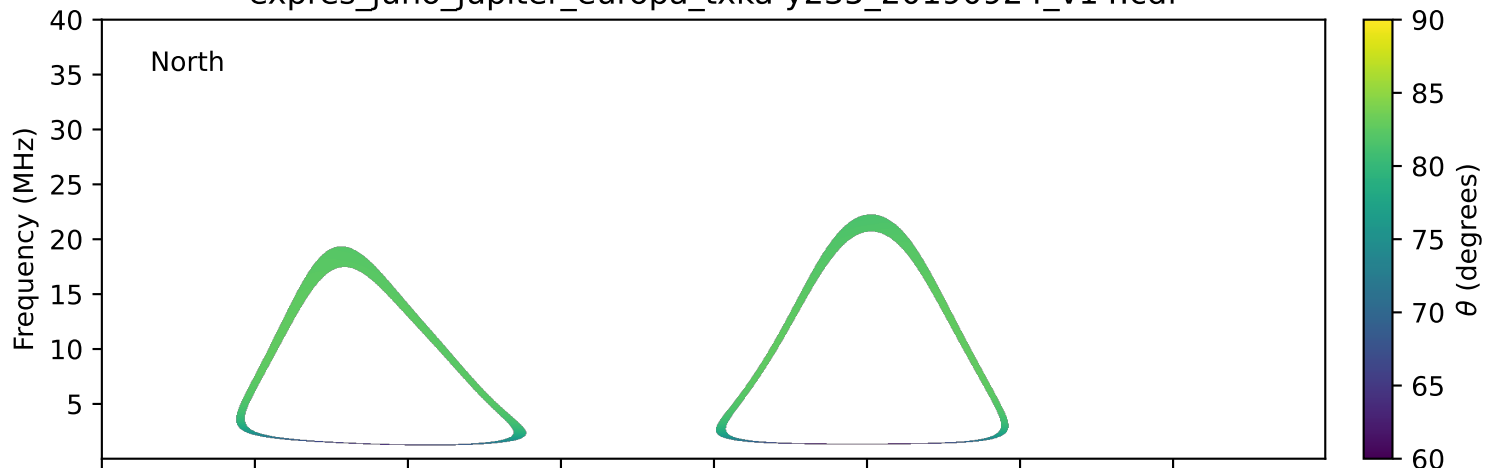
expres_juno_jupiter_europa_txka-y235_20190924_v14.cdf
