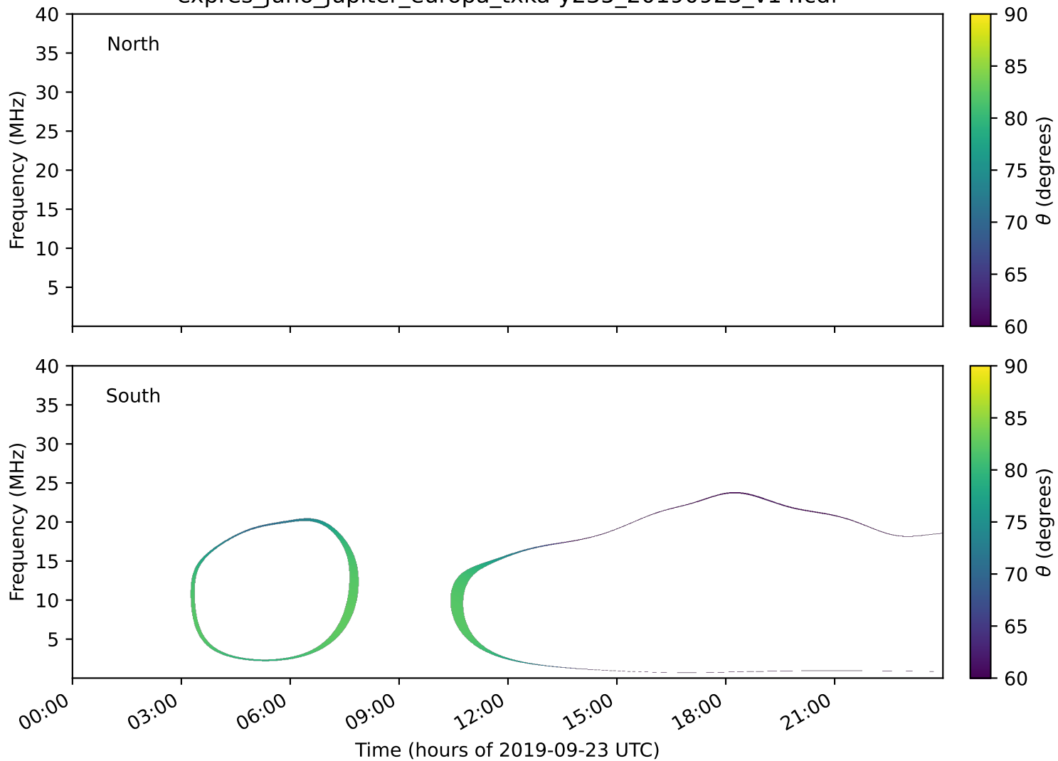
expres_juno_jupiter_europa_txka-y235_20190923_v14.cdf
