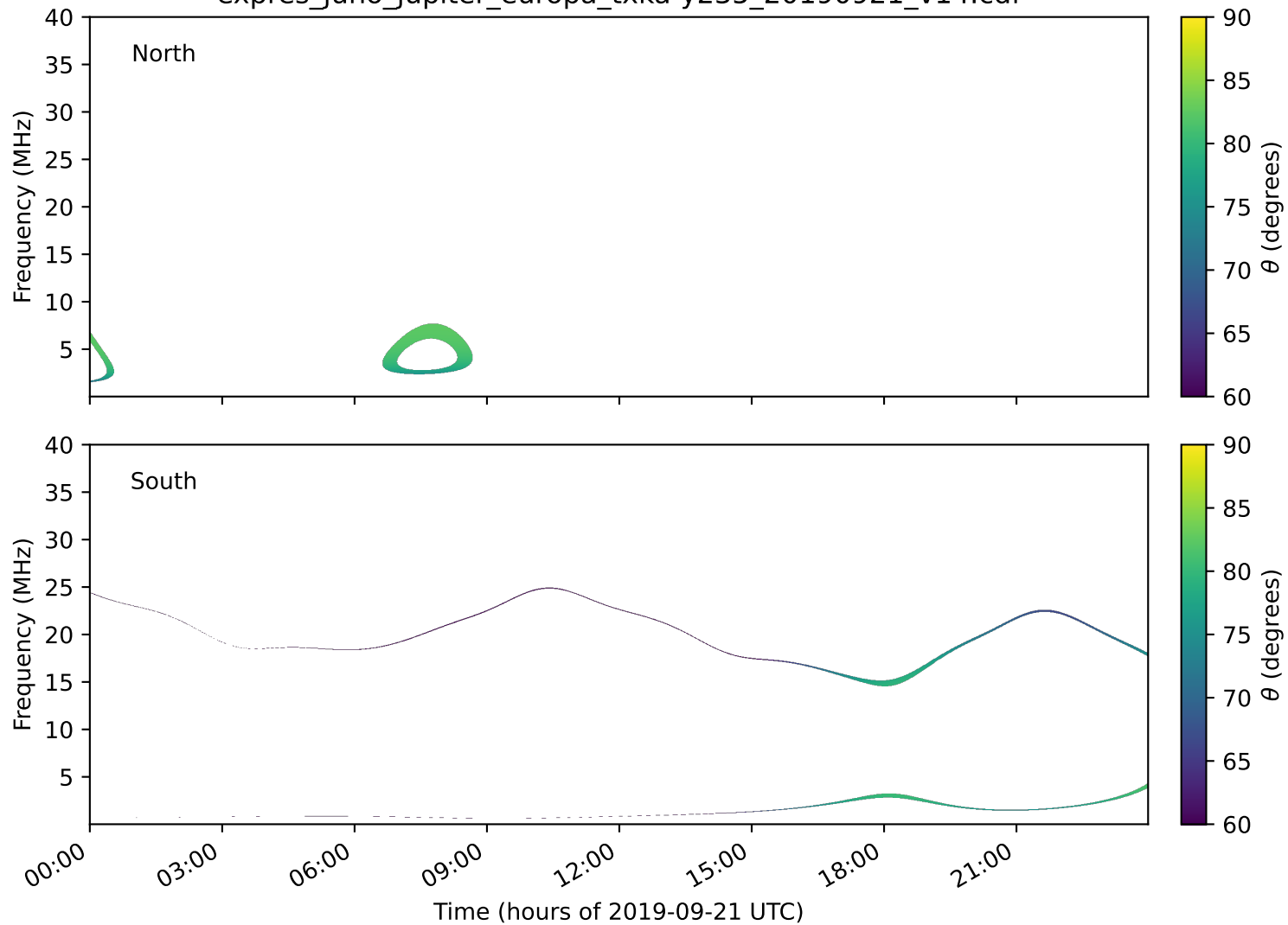
expres_juno_jupiter_europa_txka-y235_20190921_v14.cdf
