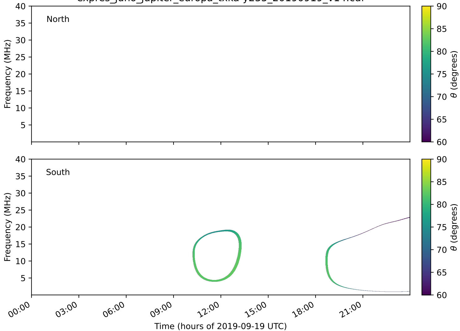
expres_juno_jupiter_europa_txka-y235_20190919_v14.cdf
