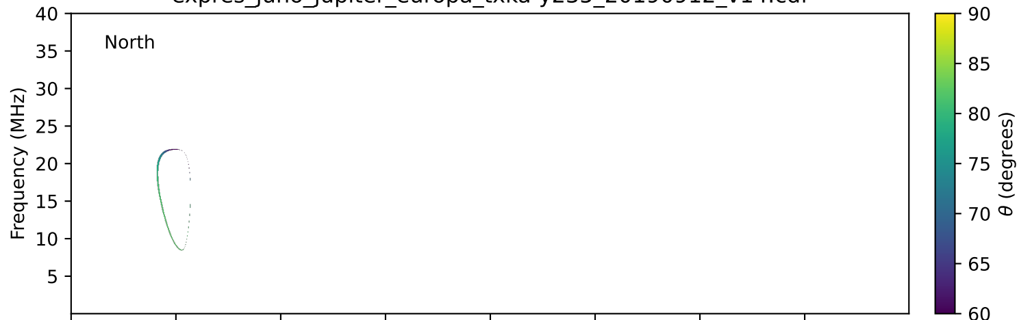
expres_juno_jupiter_europa_txka-y235_20190912_v14.cdf
