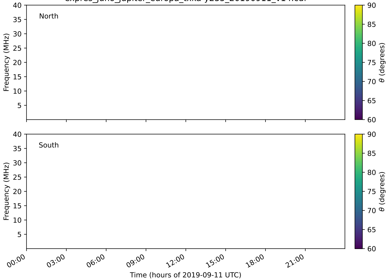
expres_juno_jupiter_europa_txka-y235_20190911_v14.cdf
