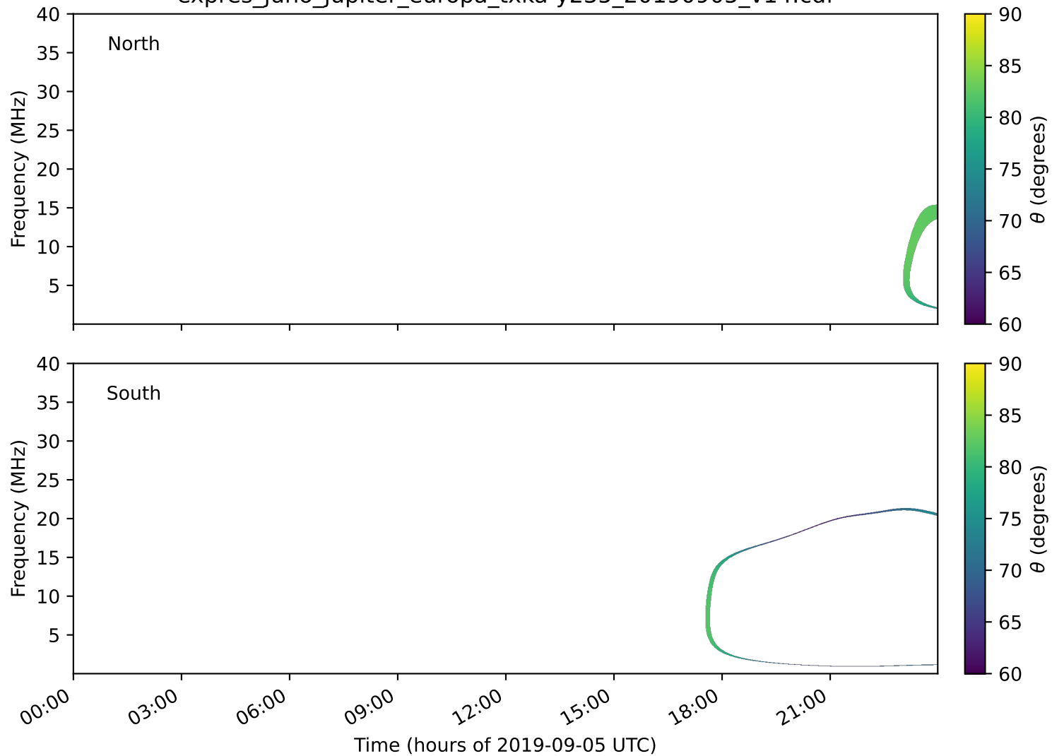
expres_juno_jupiter_europa_txka-y235_20190905_v14.cdf
