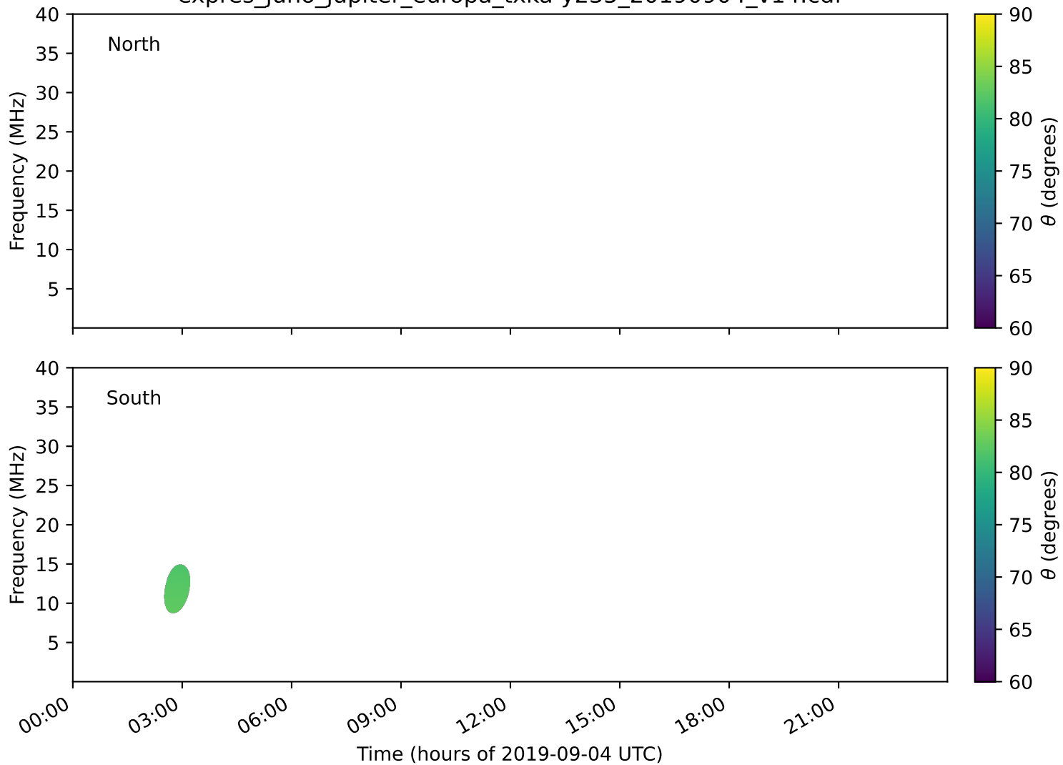
expres_juno_jupiter_europa_txka-y235_20190904_v14.cdf
