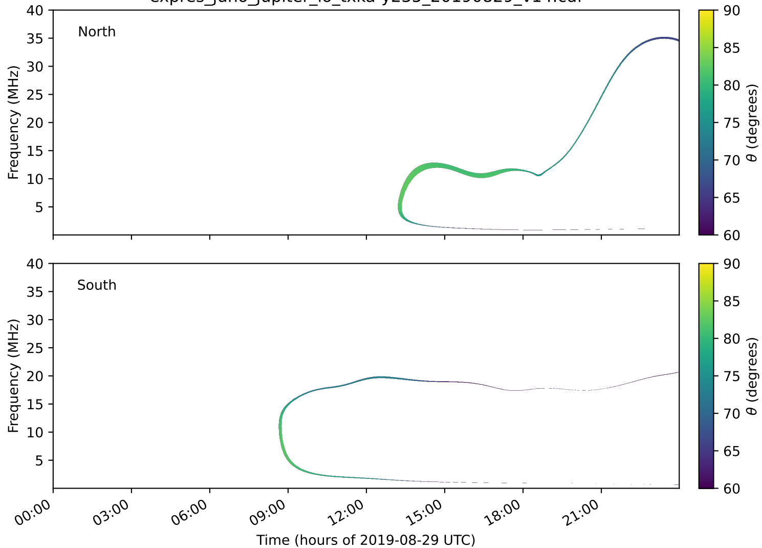
expres_juno_jupiter_io_txka-y235_20190829_v14.cdf
