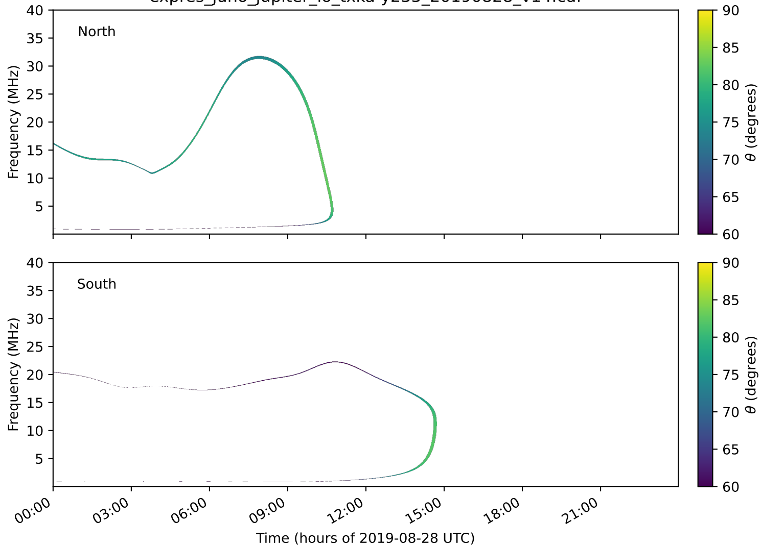
expres_juno_jupiter_io_txka-y235_20190828_v14.cdf
