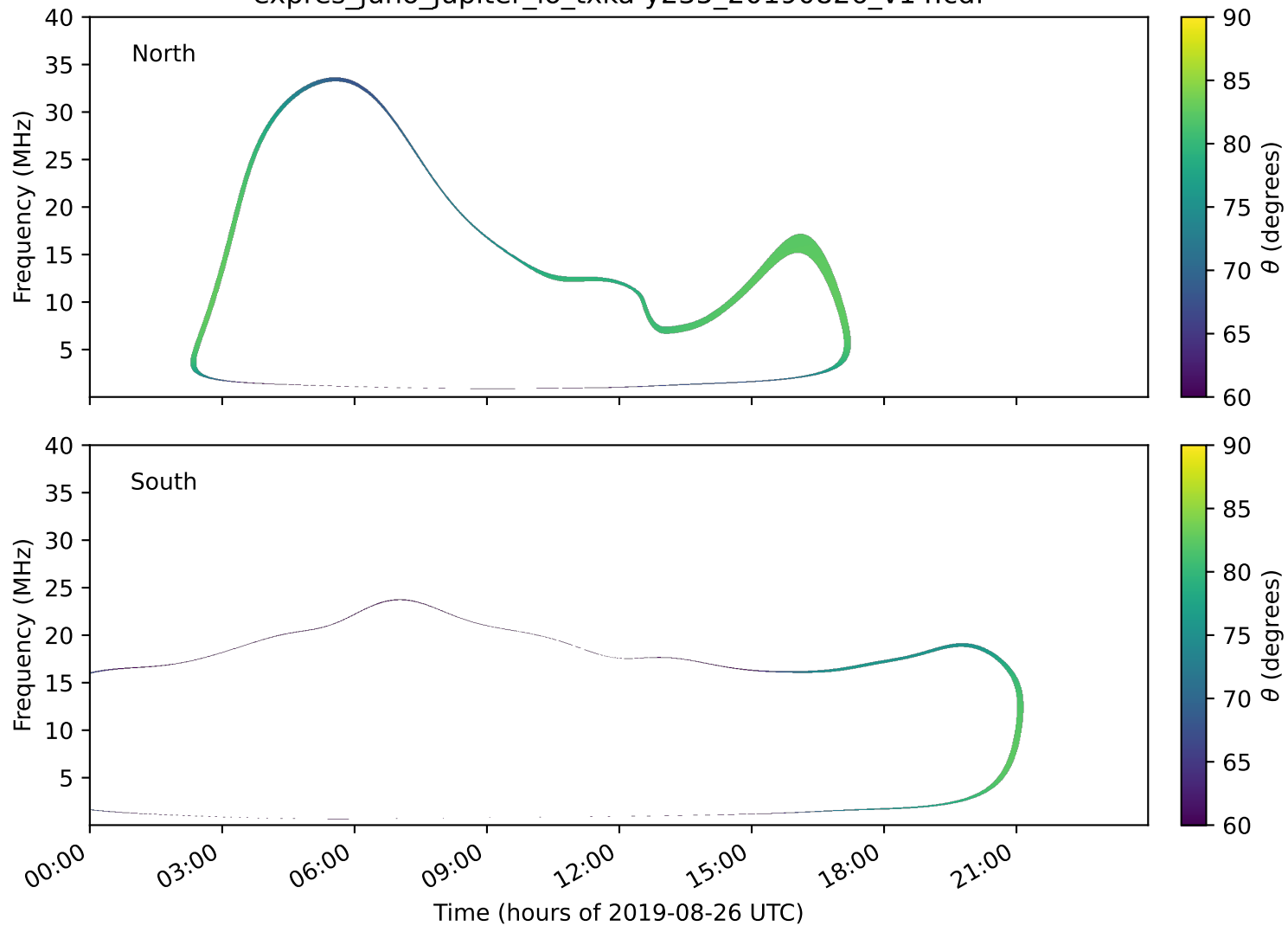
expres_juno_jupiter_io_txka-y235_20190826_v14.cdf
