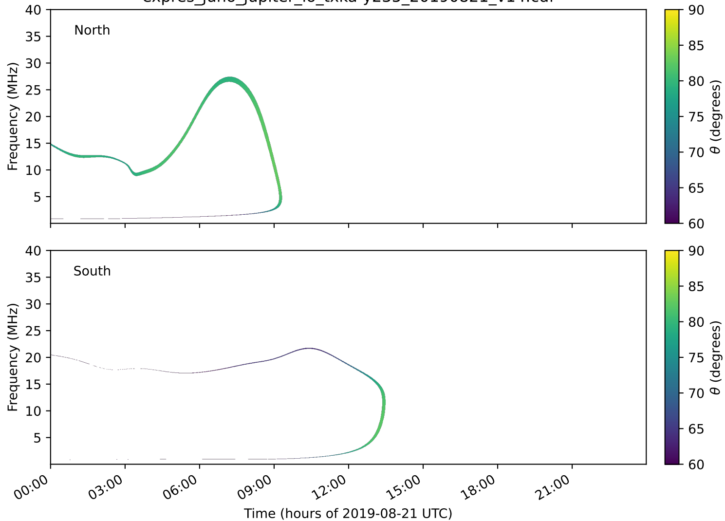
expres_juno_jupiter_io_txka-y235_20190821_v14.cdf
