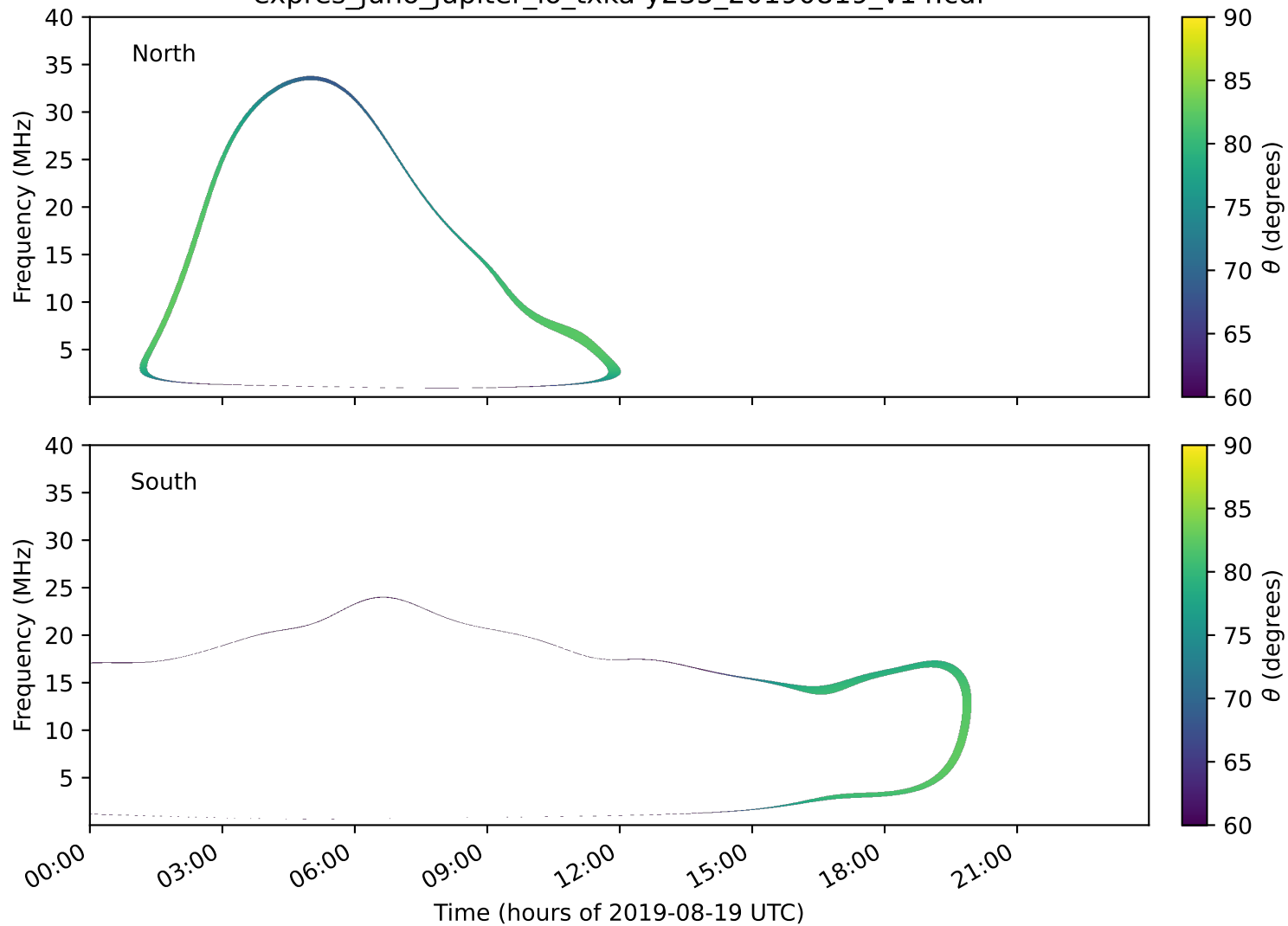
expres_juno_jupiter_io_txka-y235_20190819_v14.cdf
