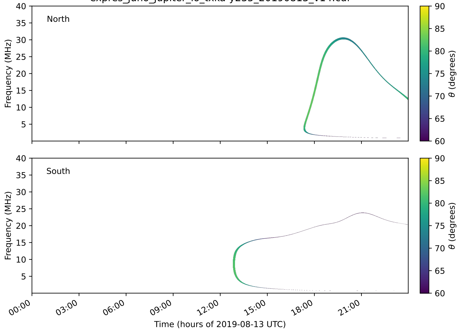
expres_juno_jupiter_io_txka-y235_20190813_v14.cdf
