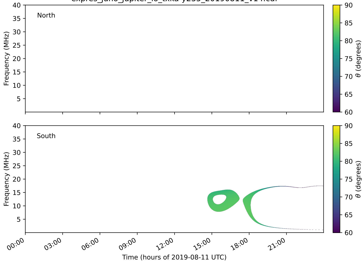
expres_juno_jupiter_io_txka-y235_20190811_v14.cdf
