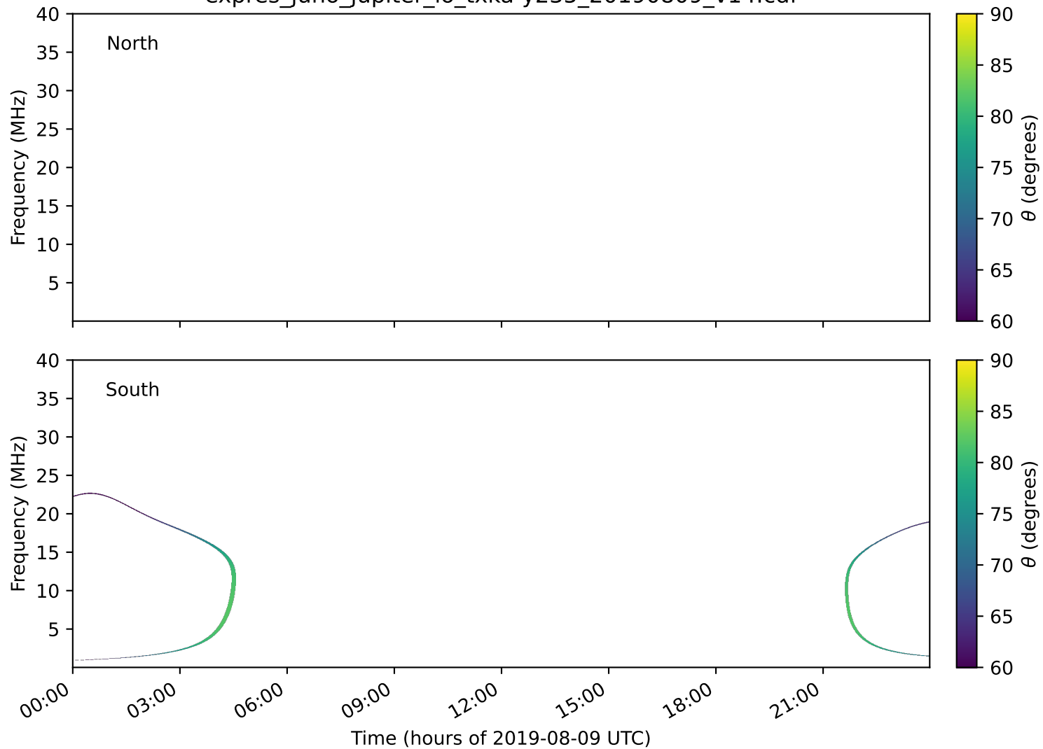
expres_juno_jupiter_io_txka-y235_20190809_v14.cdf
