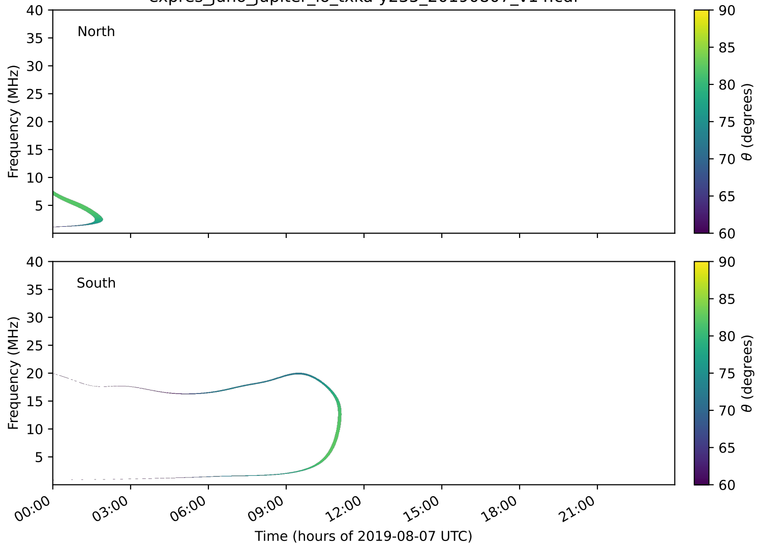
expres_juno_jupiter_io_txka-y235_20190807_v14.cdf
