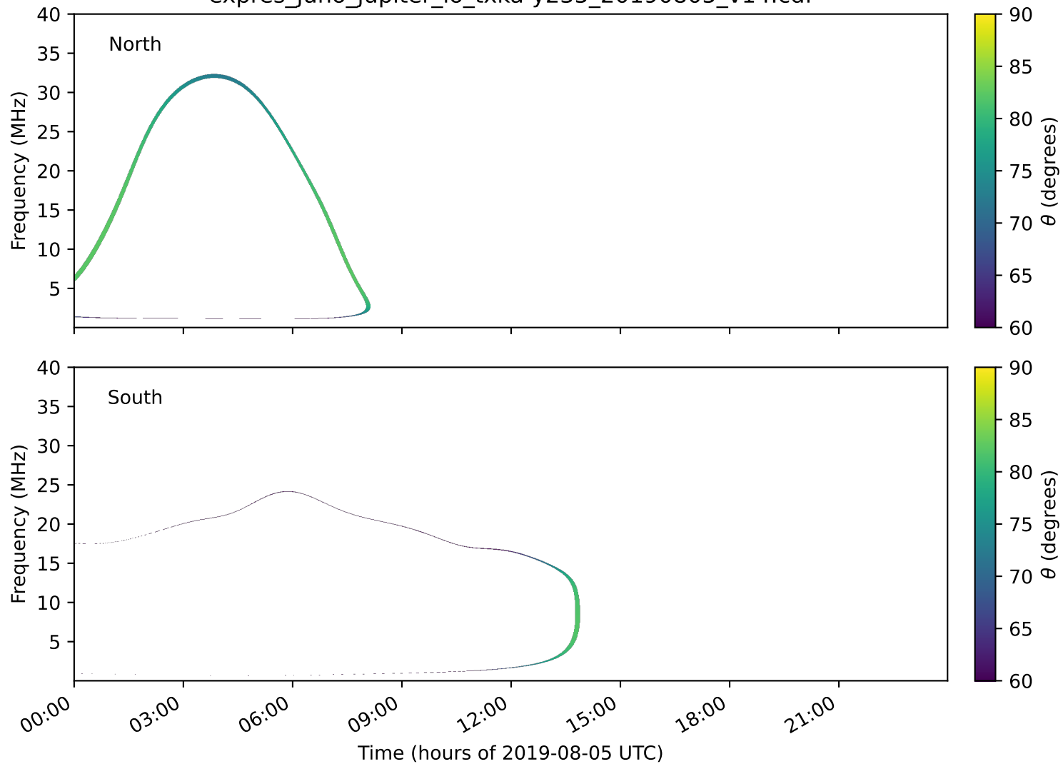
expres_juno_jupiter_io_txka-y235_20190805_v14.cdf
