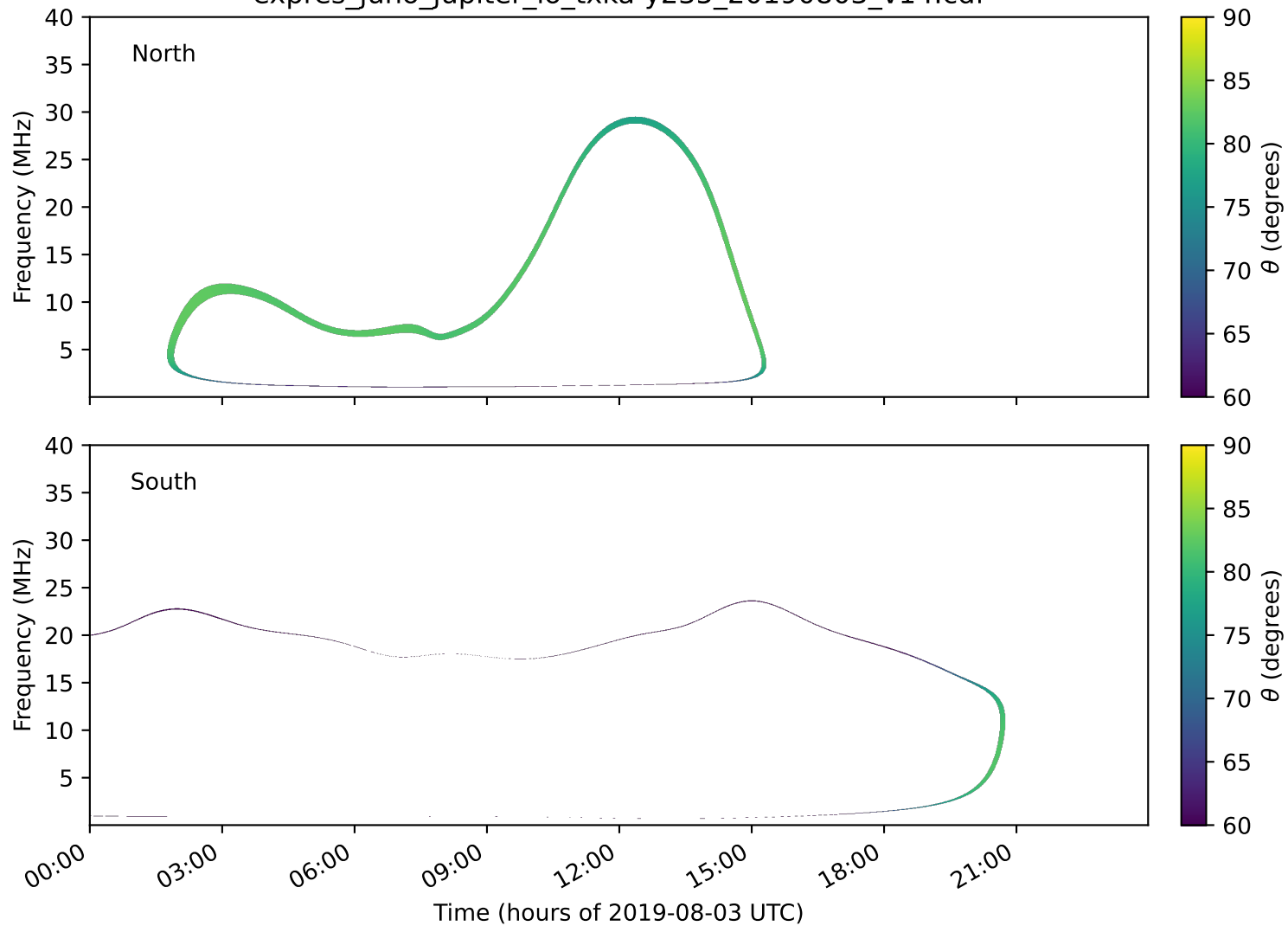
expres_juno_jupiter_io_txka-y235_20190803_v14.cdf
