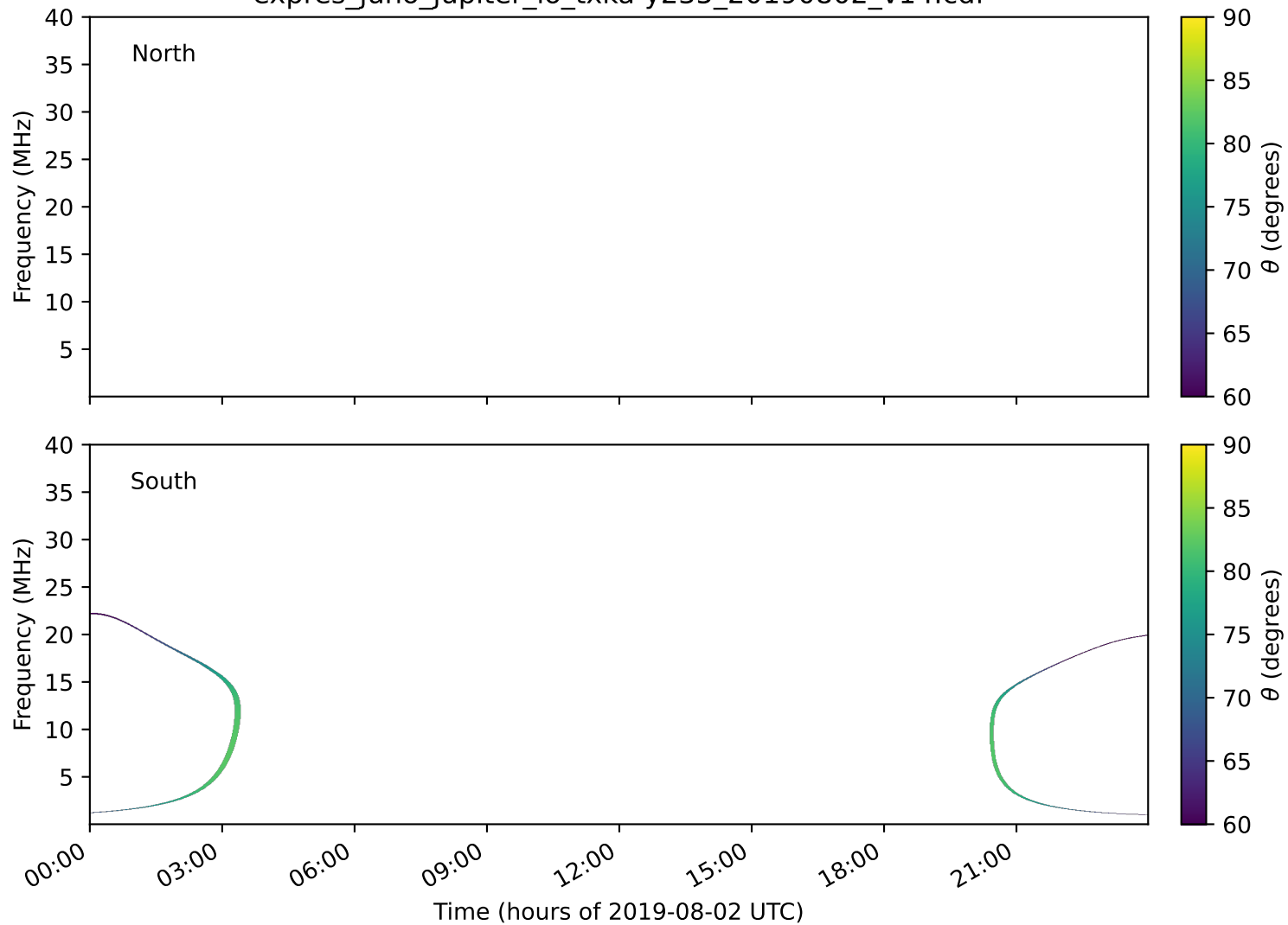
expres_juno_jupiter_io_txka-y235_20190802_v14.cdf
