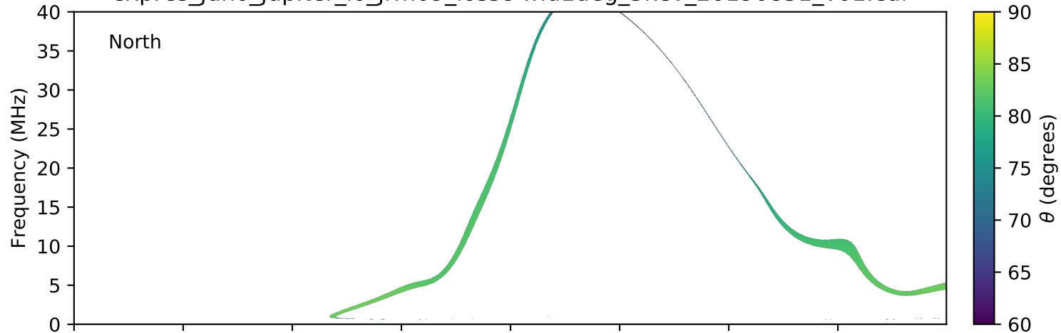
expres_juno_jupiter_io_jrm09_lossc-wid1deg_3kev_20190831_v01.cdf
