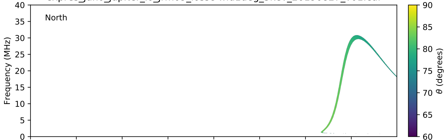
expres_juno_jupiter_io_jrm09_lossc-wid1deg_3kev_20190827_v01.cdf
