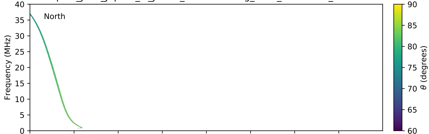
expres_juno_jupiter_io_jrm09_lossc-wid1deg_3kev_20190823_v01.cdf
