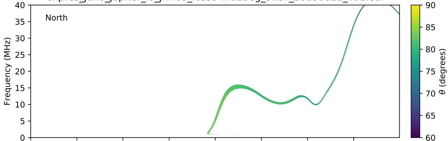
expres_juno_jupiter_io_jrm09_lossc-wid1deg_3kev_20190822_v01.cdf
