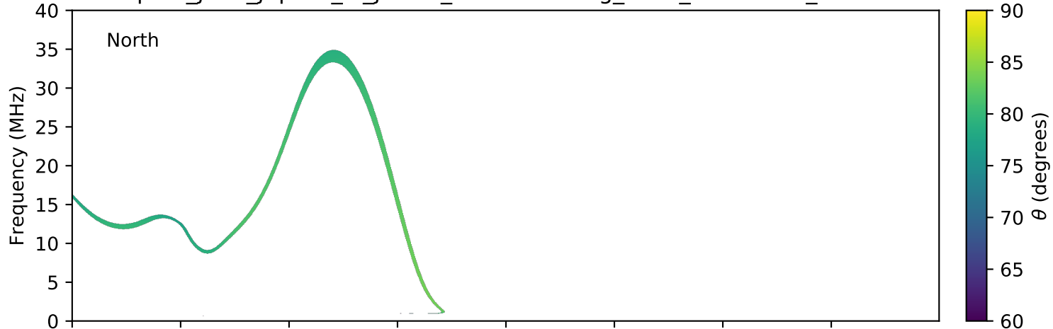
expres_juno_jupiter_io_jrm09_lossc-wid1deg_3kev_20190821_v01.cdf
