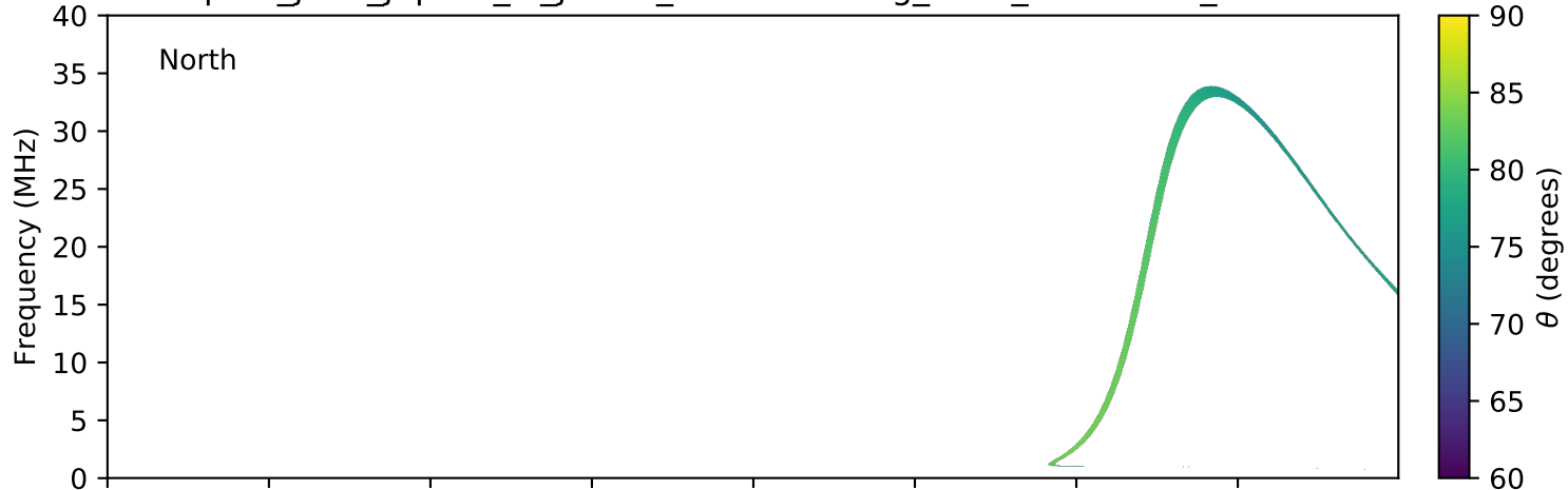
expres_juno_jupiter_io_jrm09_lossc-wid1deg_3kev_20190820_v01.cdf
