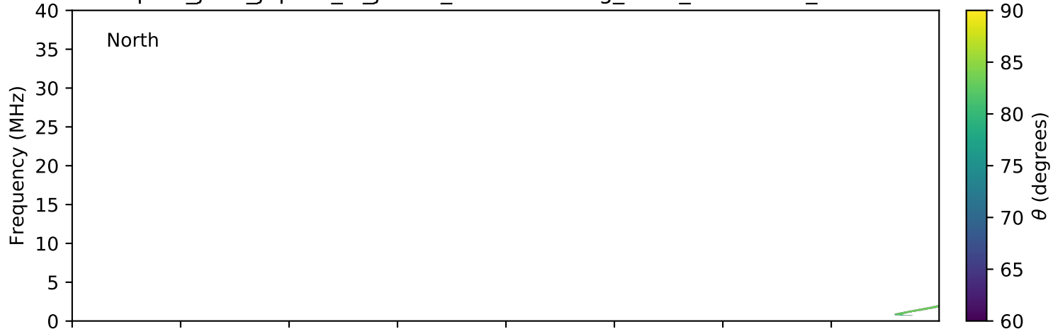
expres_juno_jupiter_io_jrm09_lossc-wid1deg_3kev_20190818_v01.cdf
