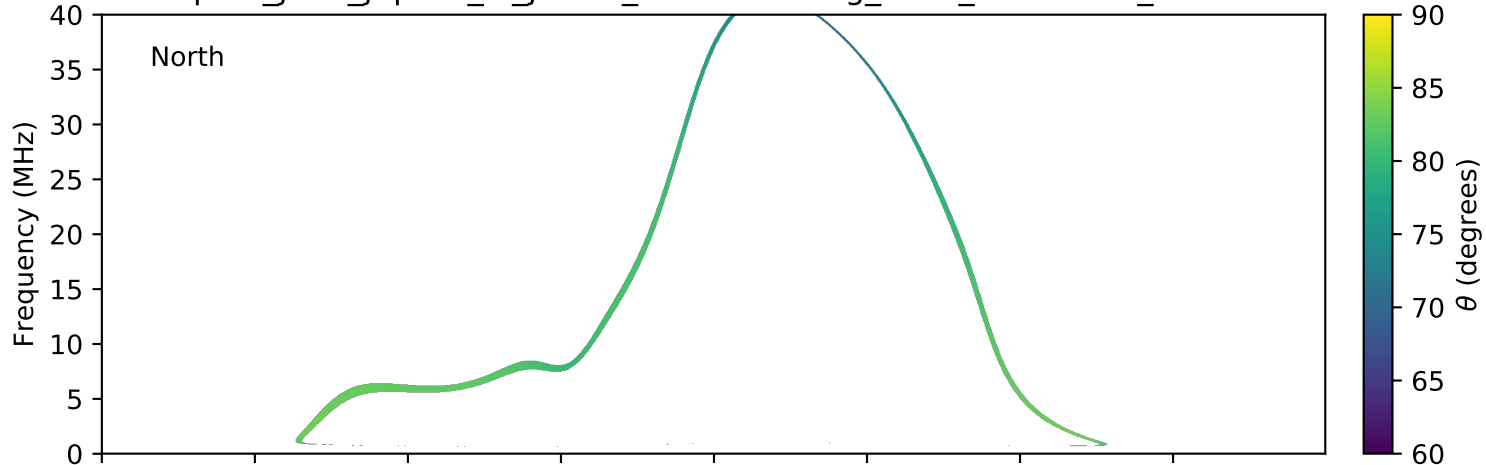
expres_juno_jupiter_io_jrm09_lossc-wid1deg_3kev_20190817_v01.cdf
