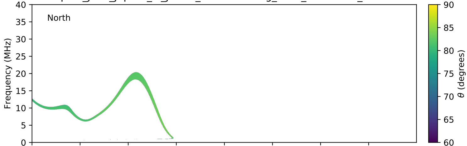
expres_juno_jupiter_io_jrm09_lossc-wid1deg_3kev_20190814_v01.cdf
