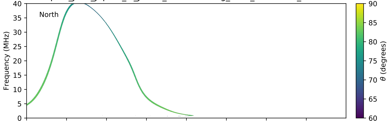
expres_juno_jupiter_io_jrm09_lossc-wid1deg_3kev_20190812_v01.cdf
