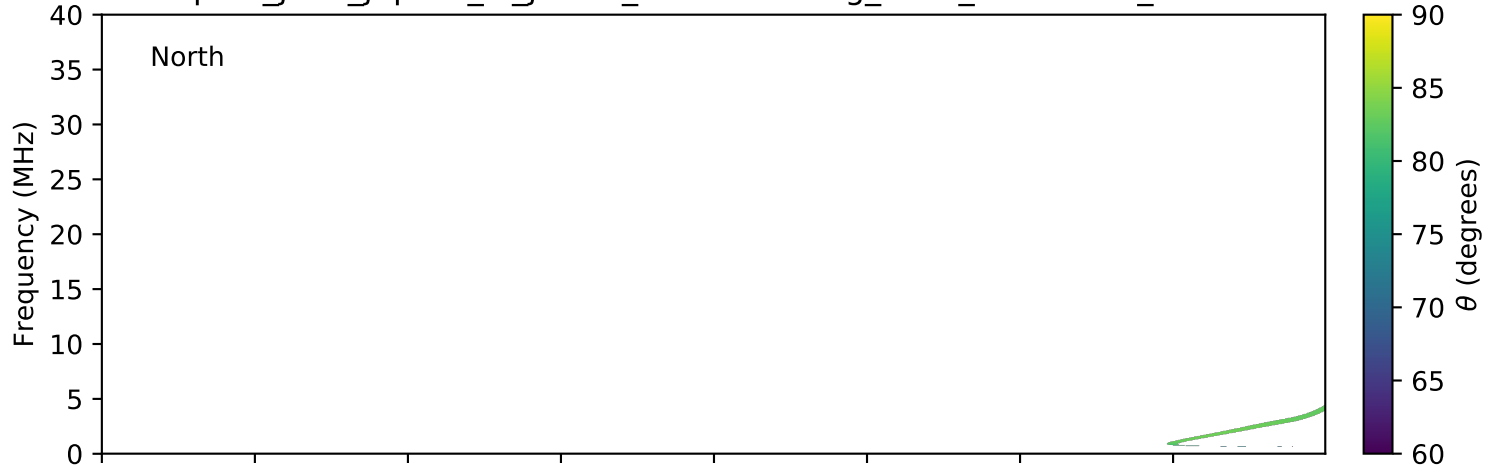
expres_juno_jupiter_io_jrm09_lossc-wid1deg_3kev_20190811_v01.cdf
