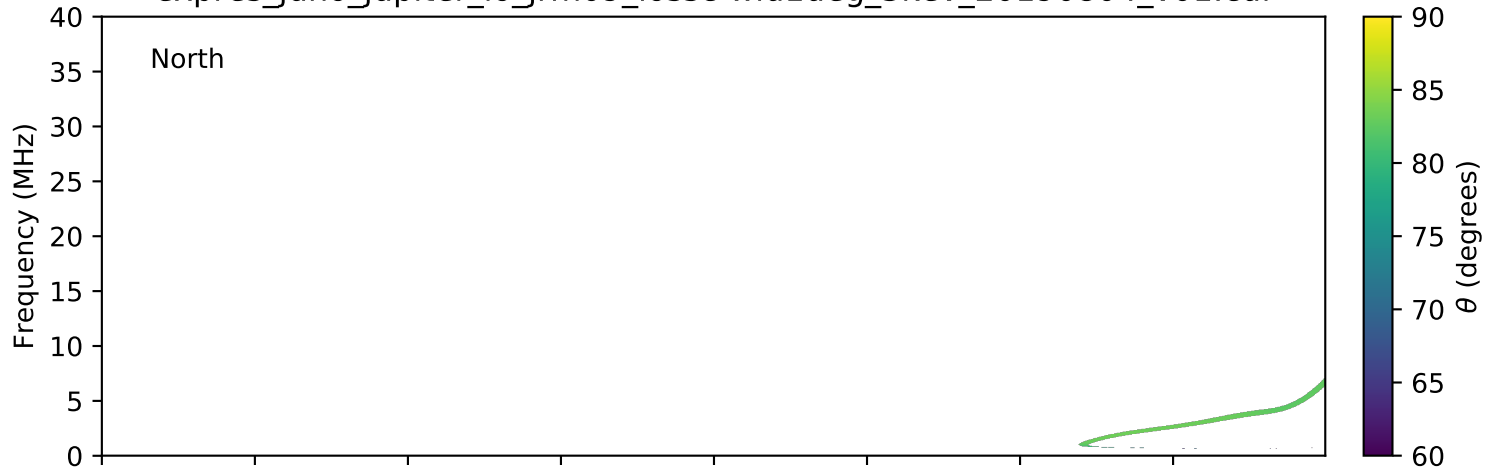
expres_juno_jupiter_io_jrm09_lossc-wid1deg_3kev_20190804_v01.cdf
