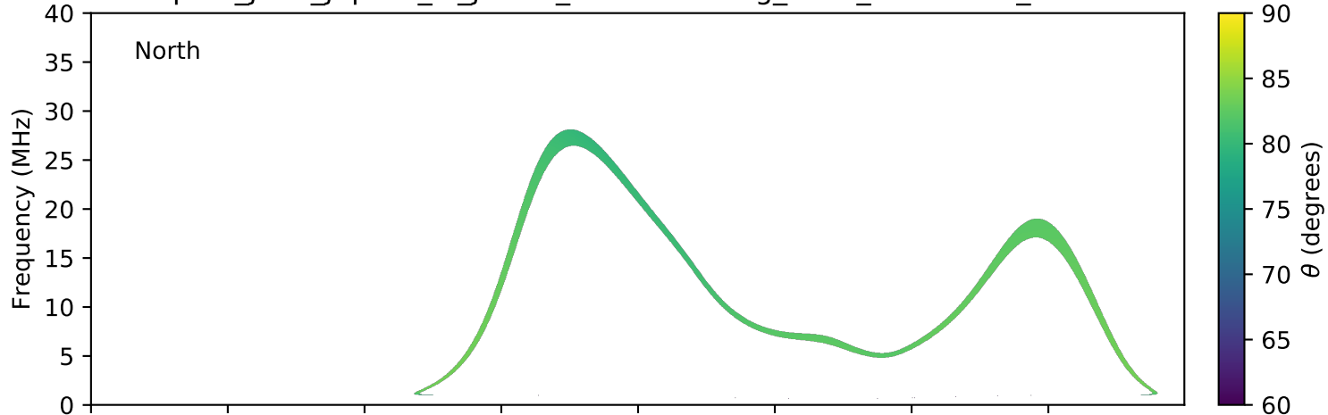
expres_juno_jupiter_io_jrm09_lossc-wid1deg_3kev_20190801_v01.cdf
