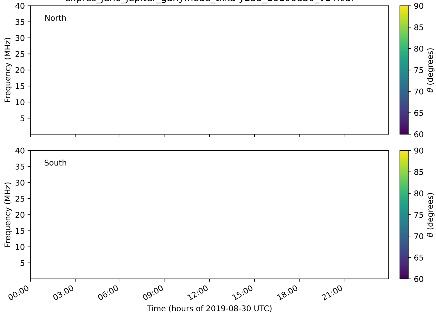
expres_juno_jupiter_ganymede_txka-y235_20190830_v14.cdf
